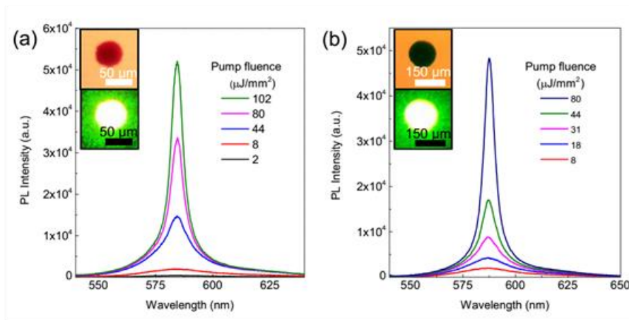
Emission spectra of a 50 μm (a) and 140 μm (b) diameter sphere under various pump pulse fluences, respectively.
