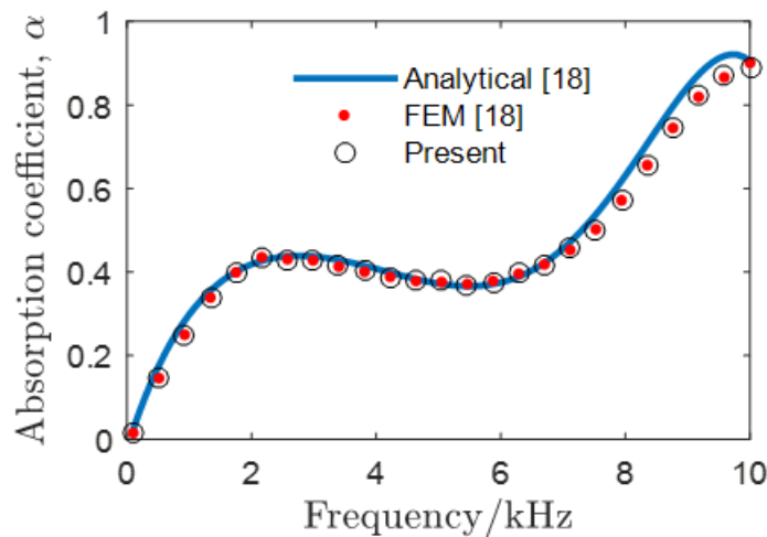
Comparison of absorption coefficients for validation of the proposed FEM.
