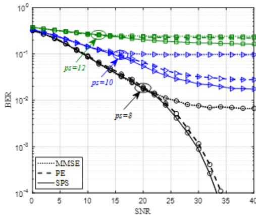
BER simulation results for the UWA-OFDM system with (a) 8PSK and (b) 16QAM on the criterion of pilot spacing p_s = 8, 10, 12
