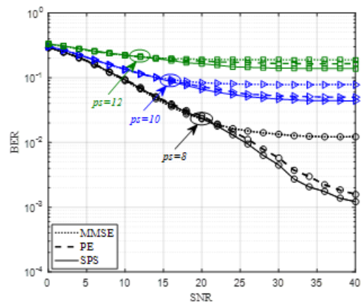
BER simulation results for the UWA-OFDM system with (a) 8PSK and (b) 16QAM on the criterion of pilot spacing p_s = 8, 10, 12
