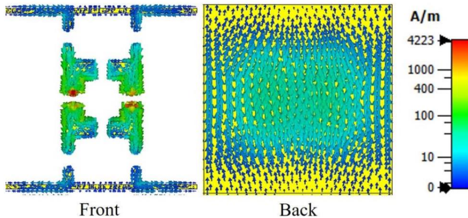
Surface-current distribution on the metamaterial absorbers at the absorption frequency of 6.4 GHz.
