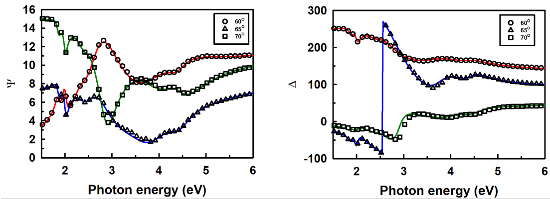
Experimental and fitting results of the polarization amplitude ratio and its phase shift at different angles.
